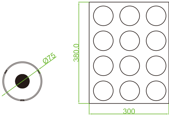
吸塑 Blister-380*300
