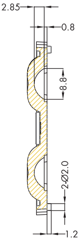
SECTION B-B
