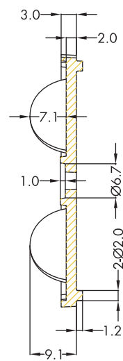
SECTION B-B
