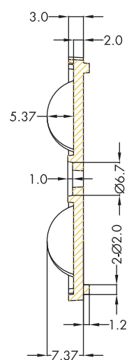
SECTION B-B
